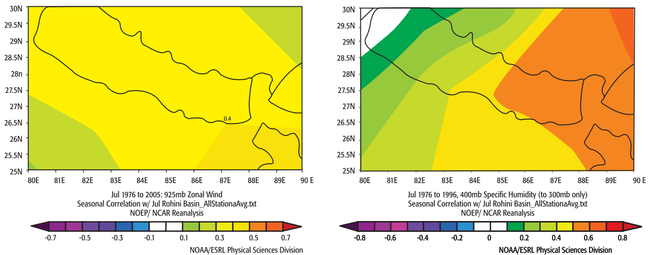
FIGURE 3 | Spatial correlations of July's (1976-2006) rainfall with zonal wind and specific humidity.
