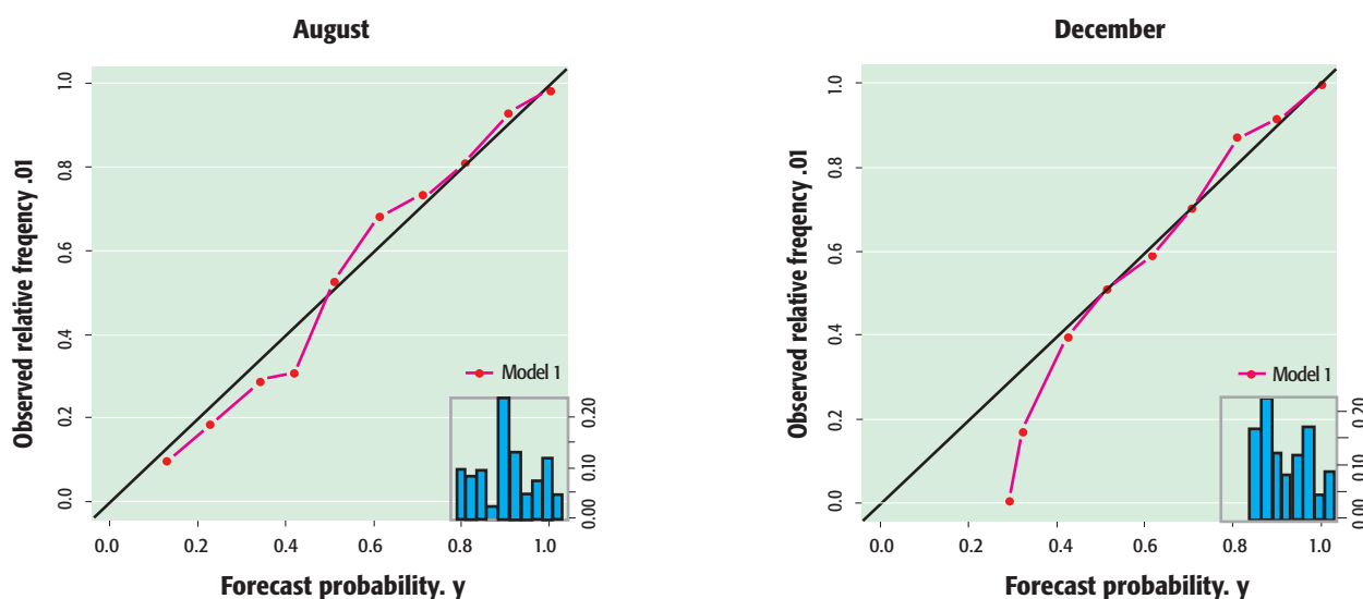
FIGURE 5 | Reliability diagrams for the months of August and December. The red line is the actual diagram and tells about the model's reliability and resolution. The histogram inset displays the sharpness (relative frequency) of the model's predictions.
