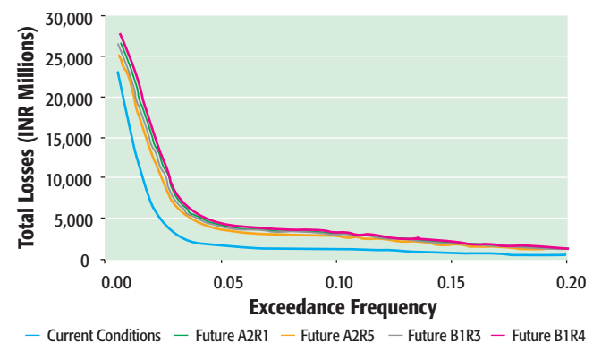
FIGURE 8 | Flood loss-frequency curves for current conditions and future climate scenarios (2007-2050)
