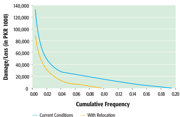
FIGURE 7 | Loss-frequency curve with relocation
