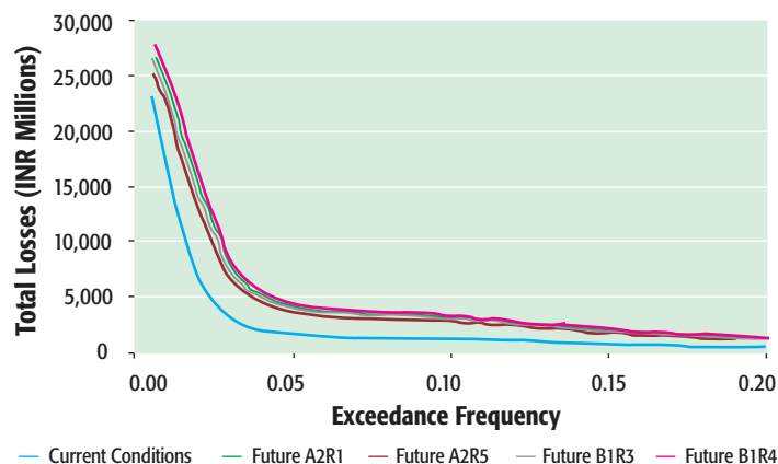
FIGURE 8 | Flood loss-frequency curves for current conditions and future climate scenarios (2007-2050) Eastern Uttar Pradesh
