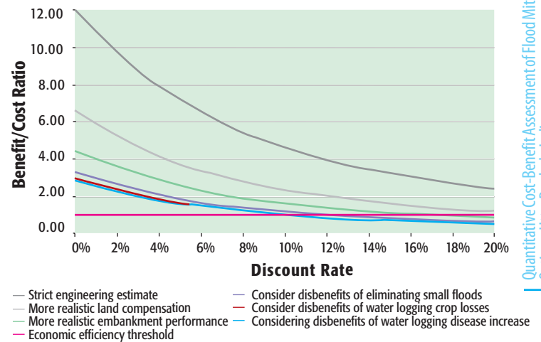
FIGURE 9 | Results of CBA for historical performance of embankments
