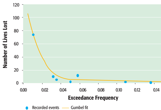
FIGURE 6 | Loss of life frequency curve for Lai floods
