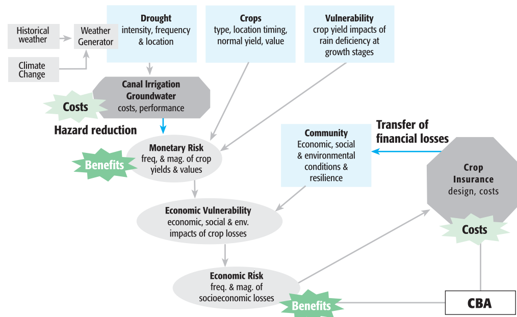
FIGURE 3 | Model algorithm
