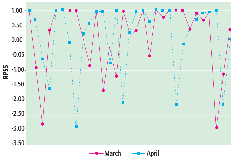
FIGURE 6 | Oscillatory behaviour of the RPSS for the months of March and April. This indicates that the historical rainfall datasets were not of sufficient length.
