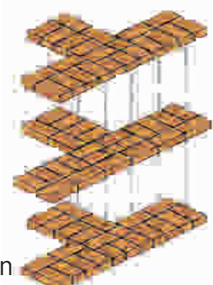
340mm (13 1/2 ") Wall
