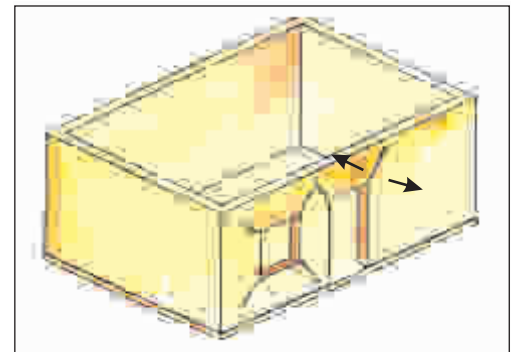
Diagonal Crack at the corner of the window and the door Cause: Wall with openings is weak against tension in diagonal direction.
