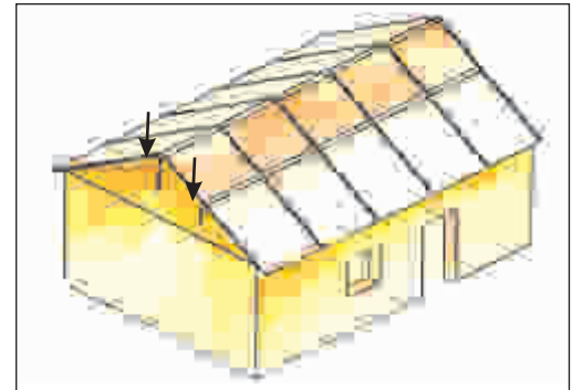
Crack under a beam Cause: Wall is unable to resist splitting tension due to concentrated load from the beam during earthquake.
