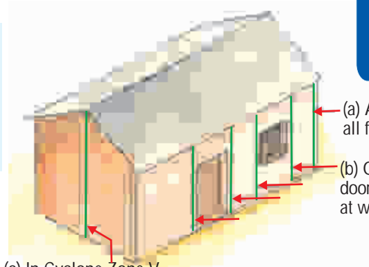
(c) In Cyclone Zone V under the ridge in gable wall
