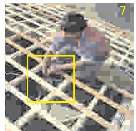
7. Pre-tension wires by twisting all wires along one diagonal together with a piece of rebar.
