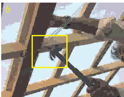
6. Tie one wire at a time around the joint of strut with rafter or purlin, stretched with carpenter's hammer.
