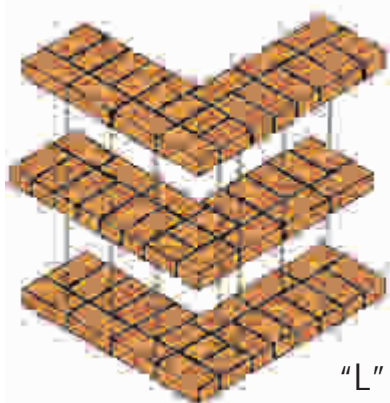
340mm (13 1/2 ") Wall
