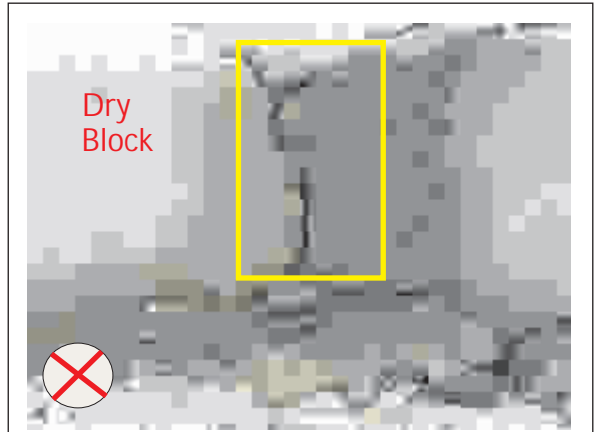
Never use Concrete Blocks in dry state in construction . It will suck the water from mortar and a crack will develop.
