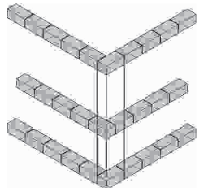
"T" Junction
