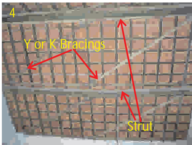
4. Install diagonal bracings starting from one end of a strut to the strut at the far end maintaining the angle close to 45 degrees, otherwise install more than one set of bracings.
