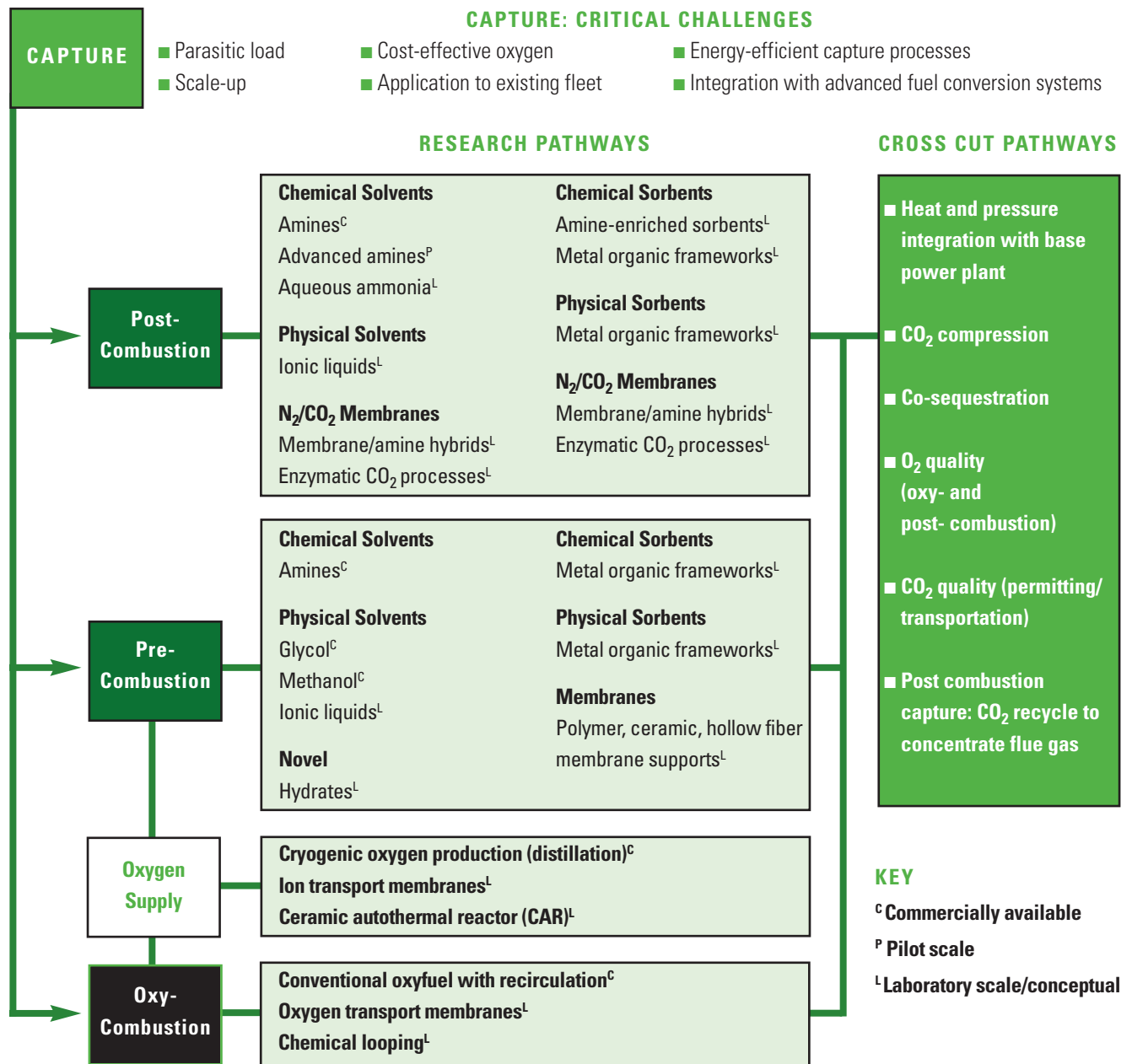
Figure 5: Critical Challenges Associated With CO 2 Capture Technologies
