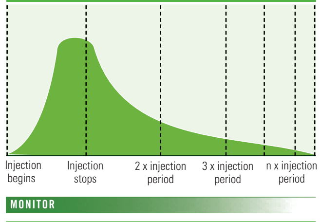
Figure 8: Conceptual Risk Profile of a Storage Project
