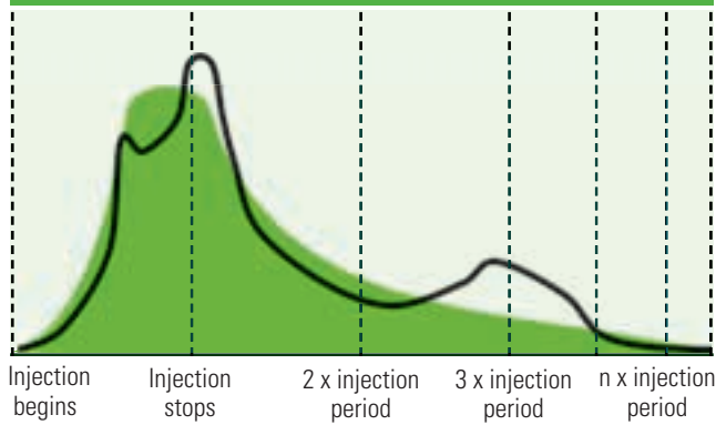
Figure 12: Conceptual Risk Profiles for a Large CCS Project Through Time
