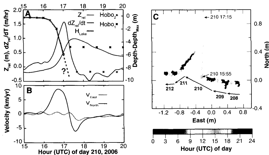
Fig. 2. Data from the 2006 lake drainage event. (A) Relative elevation ( Z_{rel} ) and rate of elevation change (left axis: black and red lines respectively) are derived from the on-shore GPS elevations smoothed to 5-min temporal resolution. Lake level as recorded by water-pressure loggers (right axis: blue and magenta stars connected with a gray line) and referenced to the lake level just before drainage. A linear fit to the last two lake-level measurements when the depth loggers remained submerged suggests that the lake drained completely by \sim 17:30 UTC (dashed gray line). (B) North (red) and east (blue) velocity components at the GPS station smoothed to 10-min temporal resolution. (C) Relative position of the GPS station during the 5 days immediately before, during, and after the drainage event showing the rapid translation of the surface as it floats up and away from the lake center, and subsequently returns. The color-bar indicates the hour of day, and the bold black arrows delineate each day's net motion.
