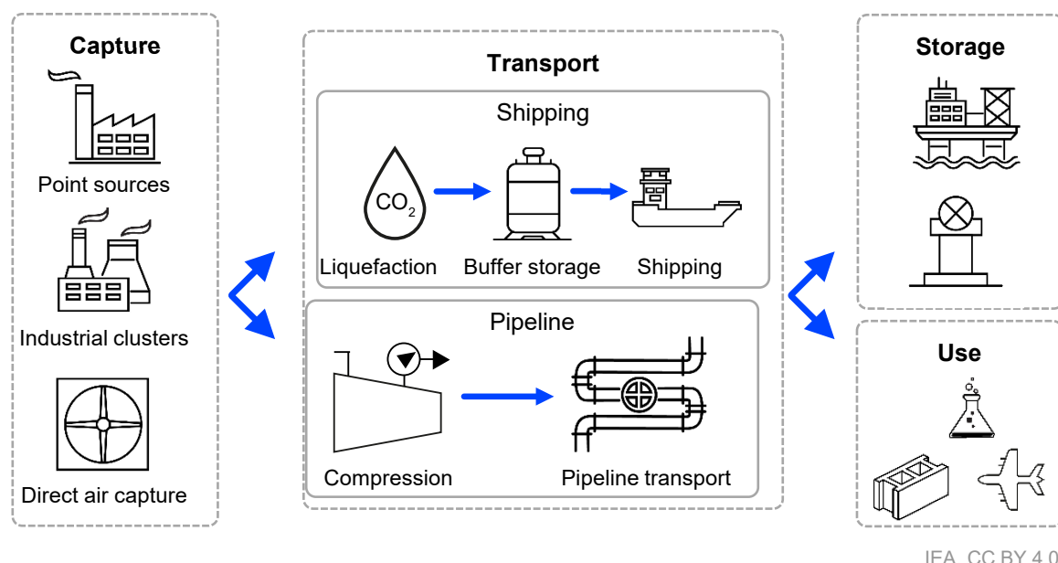
Figure 5.31 Criteria for CO 2 source-sink matching
