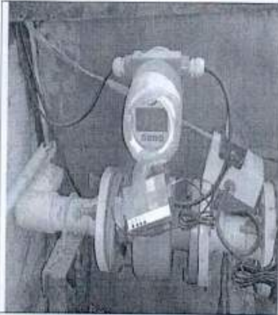
(a) Photograph of Tubewell No.1 with attached flow meter at Taj Hotel & Convention Centre, Agra.
