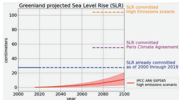
FIGURE 2-7. Committed Sea-Level Rise from Greenland at Today's and Future Emissions
