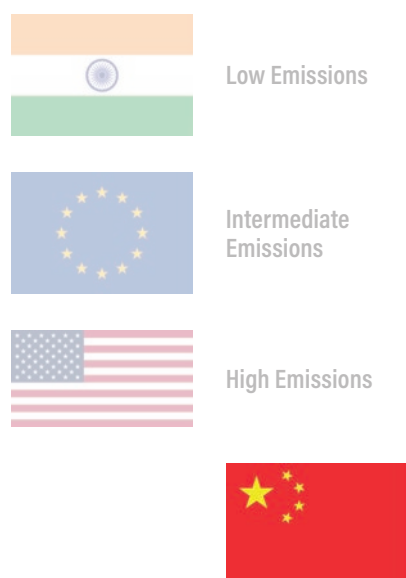
FIGURE 4-5. Permafrost Emissions at 4–5°C in 2100
