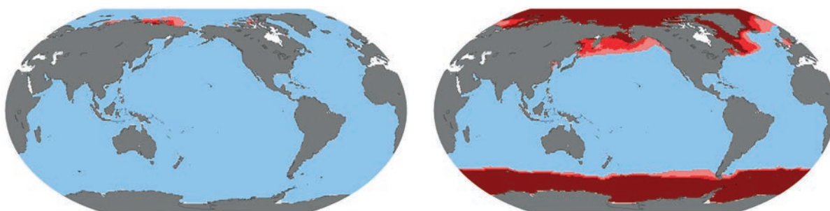
FIGURE 6-1. Acidification with Low Emissions (left) and Very High Emissions (right)
