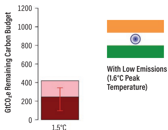
FIGURE 4-2. Permafrost Decreases Our Carbon Budget
