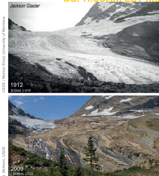
Glacier National Park: Jackson Glacier in 1912 (above) and 2009 (below)
