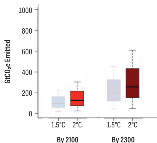
FIGURE 4-8. Multi-generational Permafrost Emissions at 2°C
