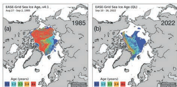
FIGURE 5-3. Multi-year Ice at Summer Minimum, 1985 and 2022
