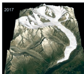
FIGURE 3-4. Great Aletsch Glacier
