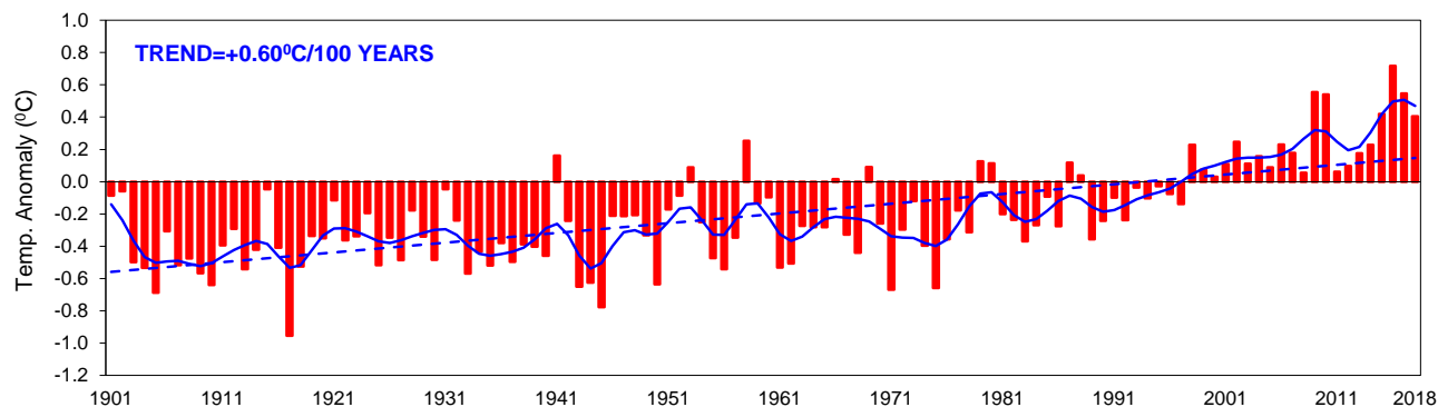
Fig.1: Annual mean land surface air temperatures anomalies averaged over India for the period 1901-2018. The anomalies were computed with respect to base period of 1981-2010. The dotted line
