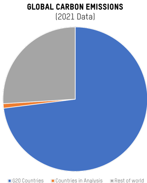
Figure 1: Global carbon emissions (2021)
