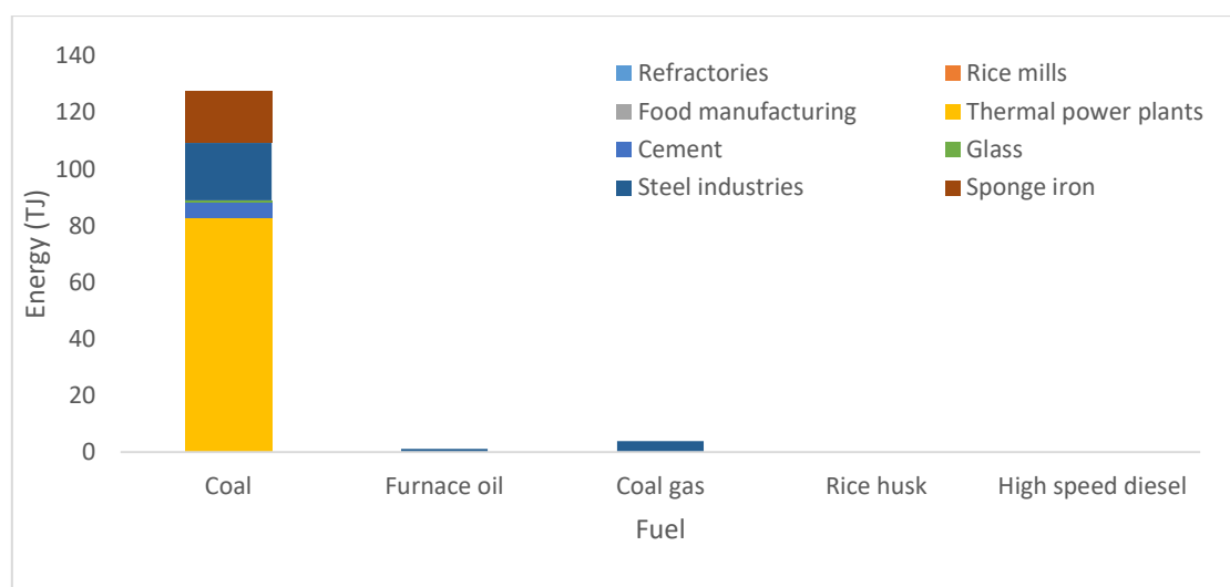
Figure 7: Total energy consumption of the industries based on their fuel usage
