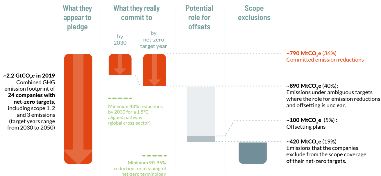
Figure 2: Net-zero pledges break down to only moderate emission reductions
