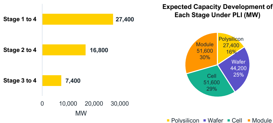
Figure 10: Cumulative Manufacturing Capacities Under Both Tranches of PLI, by PV Manufacturing Stages
