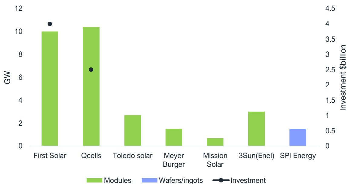
Figure 14: Proposed Expansion Plans of Solar PV Module Manufacturers in the U.S.
