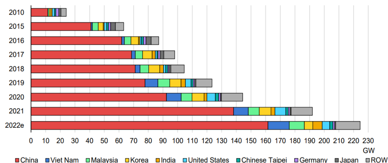
Figure 13: Global Solar PV Module Production, 2010-2022
