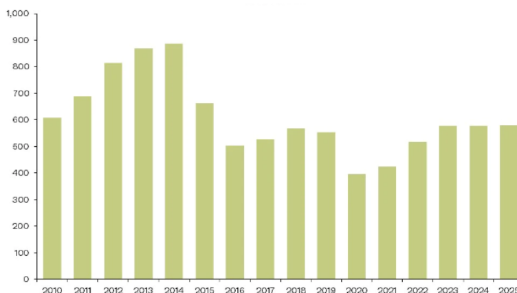
Figure 1.17 • Global upstream investments in oil and gas, 2010–26 ($ billion)
