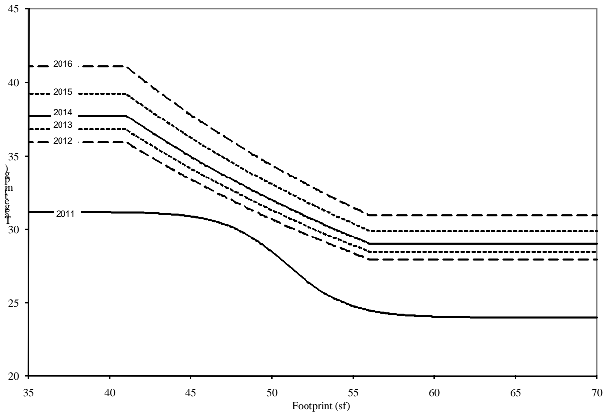
Figure IV.A.5-1 Final MY 2011 and Final MY 2012-2016 Passenger Car Fuel Economy Targets
