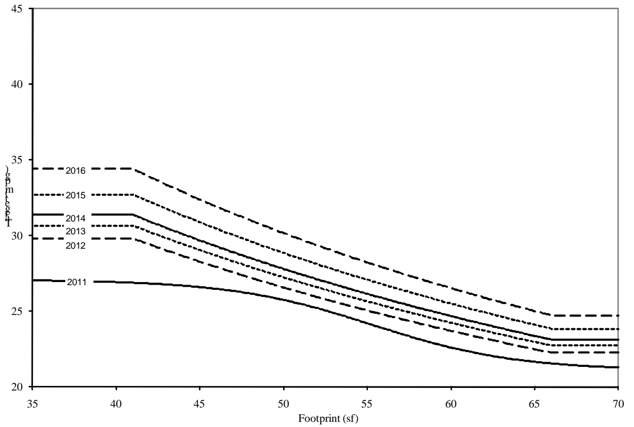
Figure IV.A.5-2 Final MY 2011 and Final MY 2012-2016 Light Truck Fuel Economy Targets
