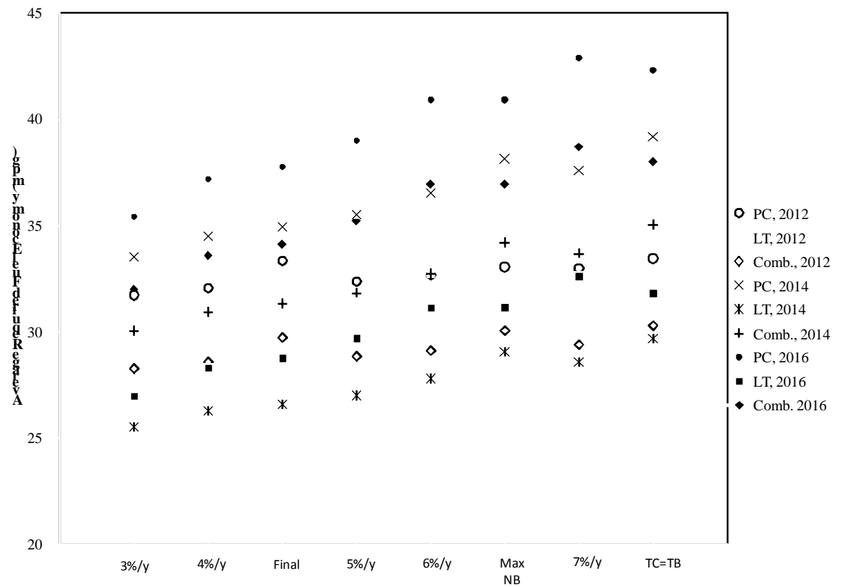
Figure IV.F-1 Average Estimated Required Fuel Economy (MYs 2012, 2014, and 2016)
