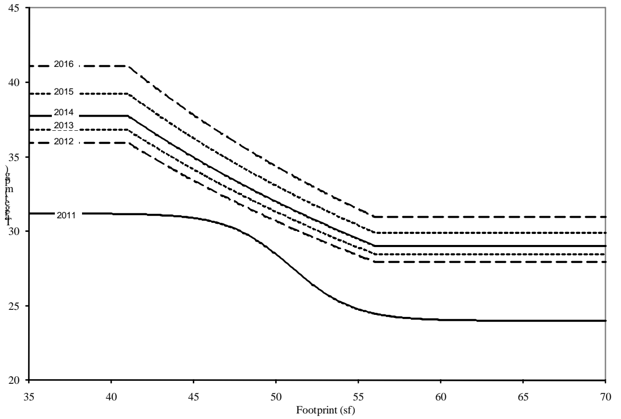
Figure IV.E.2-1 Final MY 2011 and Final MY 2012-2016 Fuel Economy Target Curves for Passenger Cars
