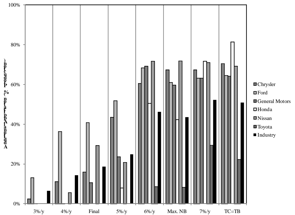
Figure IV.F-4 Additional Application of Engine Turbocharging & Downsizing (MY 2016)
