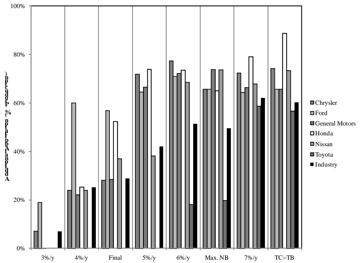
Figure IV.F-3 Additional Application of GDI (MY 2016)
